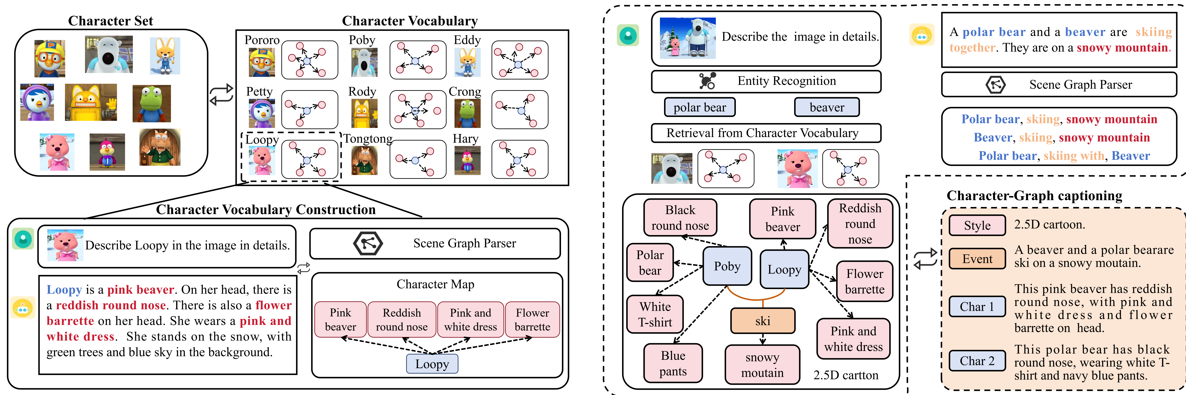
(a) Character-Graph construction with character vocabulary(left side) and captioning into semantic-rich text(right side).
